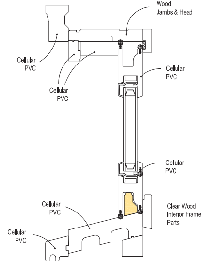
Legend Double Hung Picture
