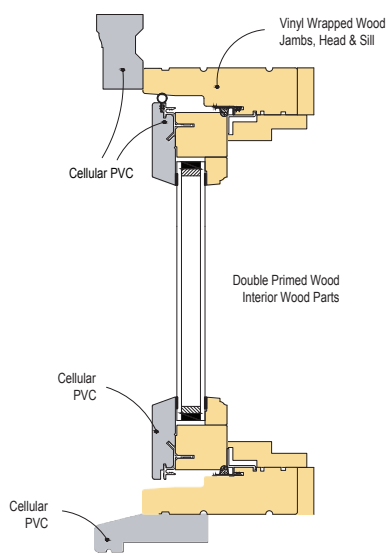
Legend Double Hung Transom
