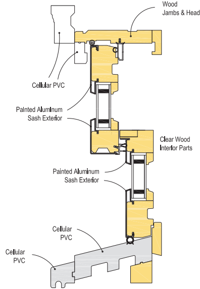
Legend HBR Double Hung
