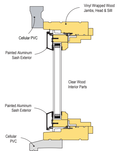
Legend HBR Double Hung Transom
