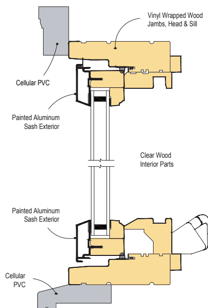
Legend HBR Casement
